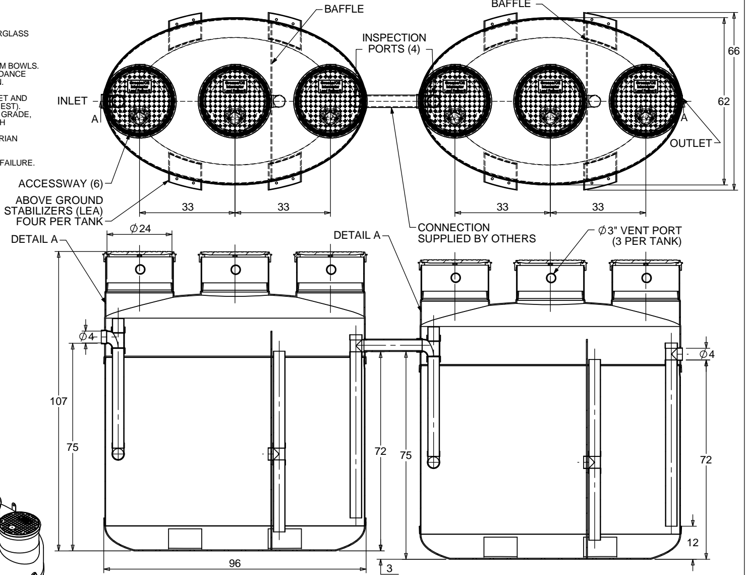
SECTION A-A SCALE 1 : 35 FOR UPC/IAPMO INSTALLATIONS
