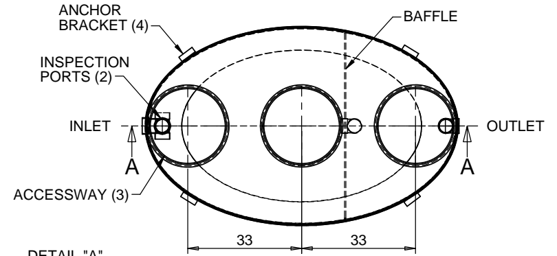
DETAIL "A" LABEL INSIDE AND OUTSIDE
