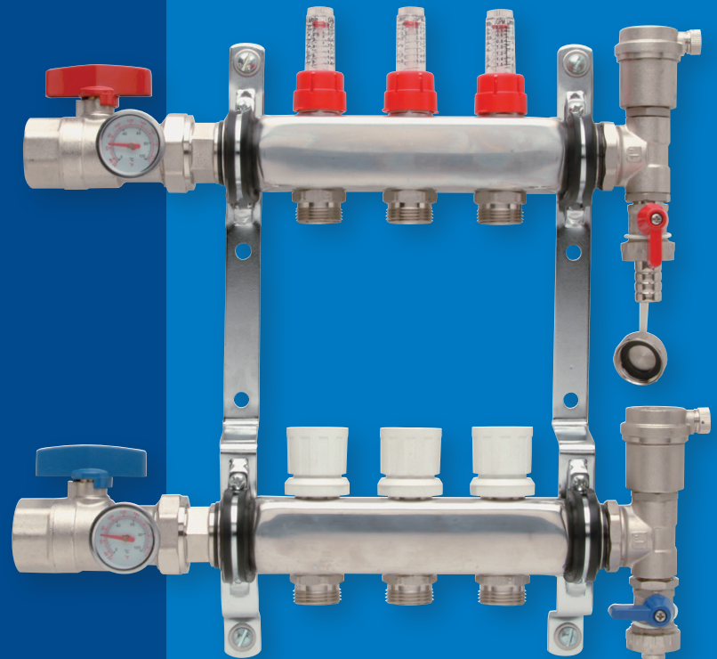
Stainless Steel Accuflow® Manifold - QHPM-3S
