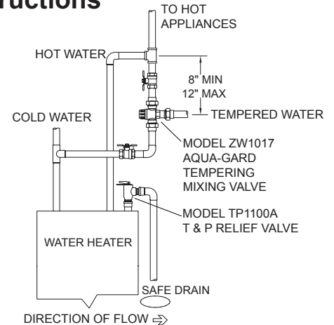
DOMESTIC WATER HEATER APPLICATION
