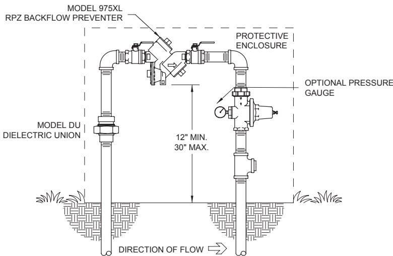
TYPICAL INSTALLATION
