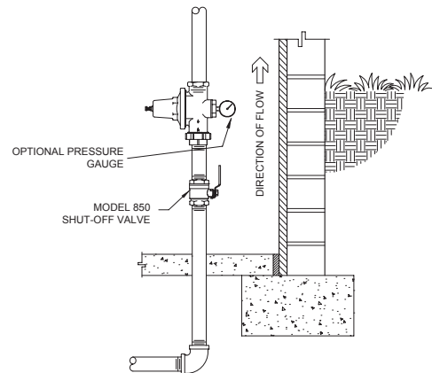
VERTICAL INSTALLATION
