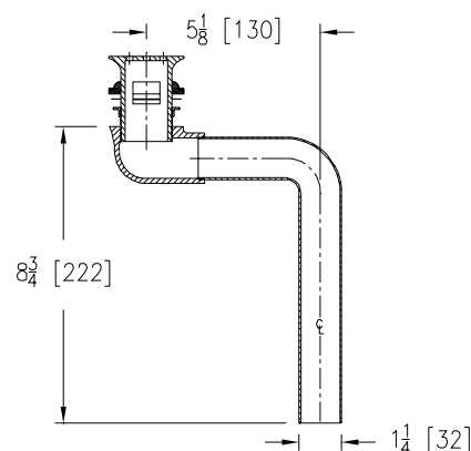
OFFSET LAVATORY STRAINER
