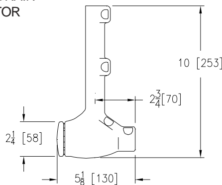
SUPPLY STOP PROTECTOR
