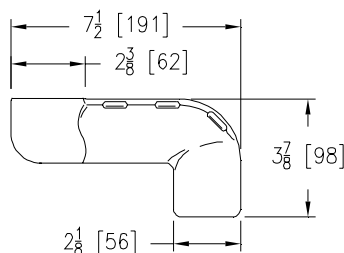
OFFSET DRAIN PROTECTOR
