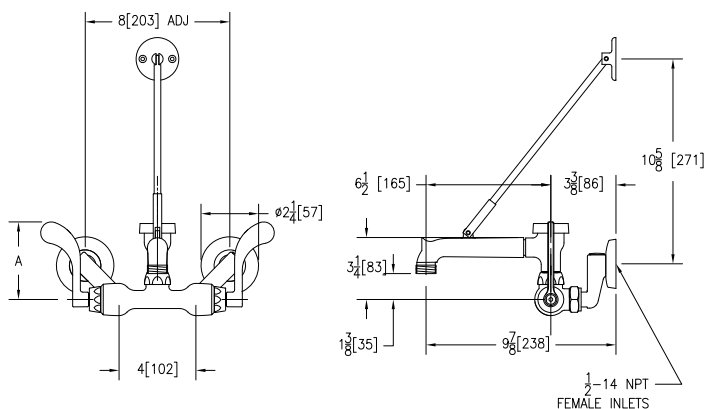
Rough-in/Overview dimensions
