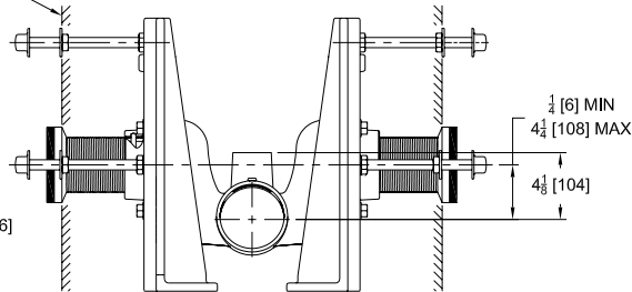
Z1201-ND4-XH Illustrated
