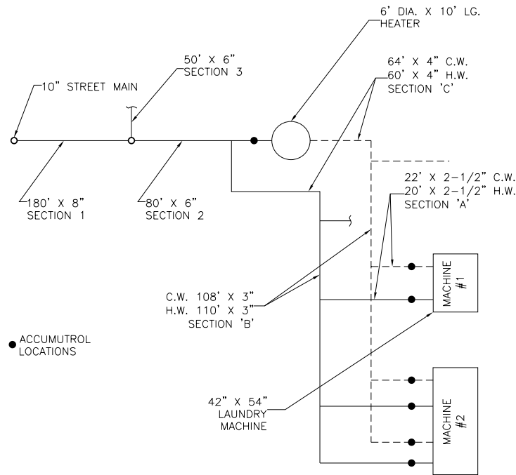
Piping Data (From Machine to Heater)
