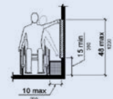
ADA Compliant Unobstructed Side Reach
