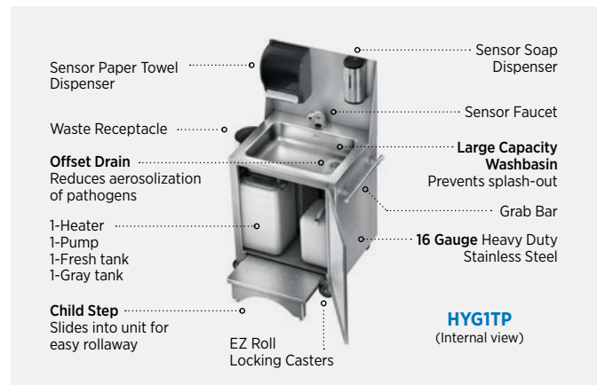
HYG1TP (Fully Accessorized Unit)
