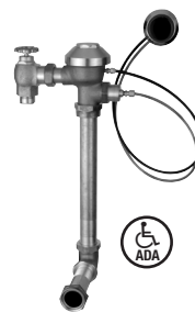
AquaVantage Exposed ZH6152AV Model With Hydraulic Actuation For Water Closets
