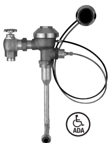
AquaVantage Exposed ZH6195AV Model With Hydraulic Actuation For 3/4" Urinals
