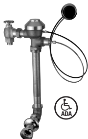
AquaVantage Exposed ZH6140AV Model With Hydraulic Actuation For Back Spud Water Closets
