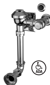
AquaVantage Exposed ZH6010AV Model With Hydraulic Actuation For Back Spud Water Closets
