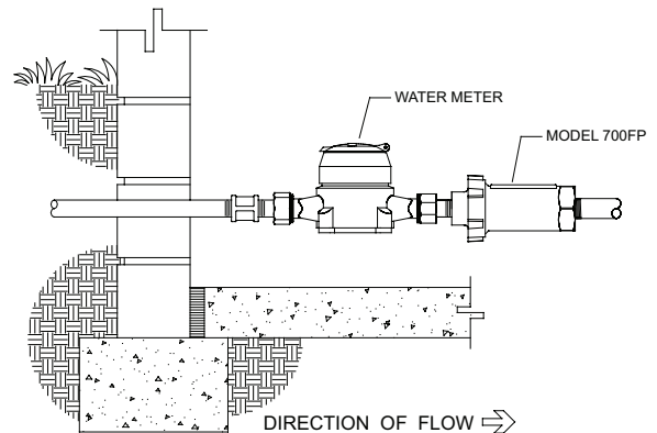
INDOOR INSTALLATION
