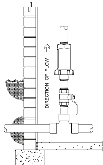
VERTICAL INSTALLATION
