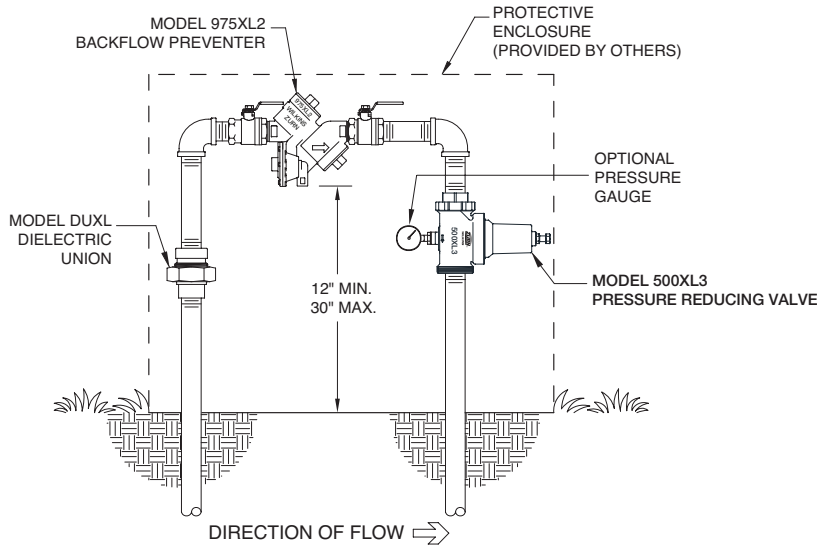
TYPICAL INSTALLATION
