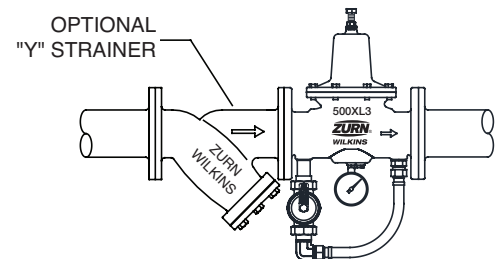
Horizontal Installation
