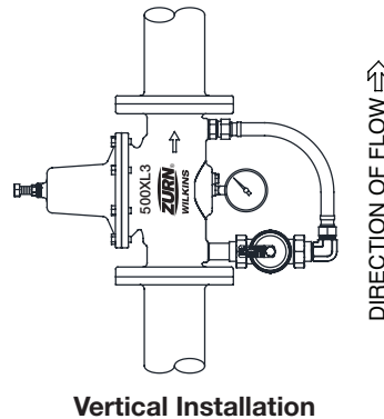
Vertical Installation
