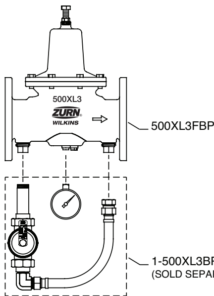
Parallel Installation
