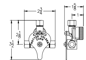
Optional P6900-MV Mixing Valve
