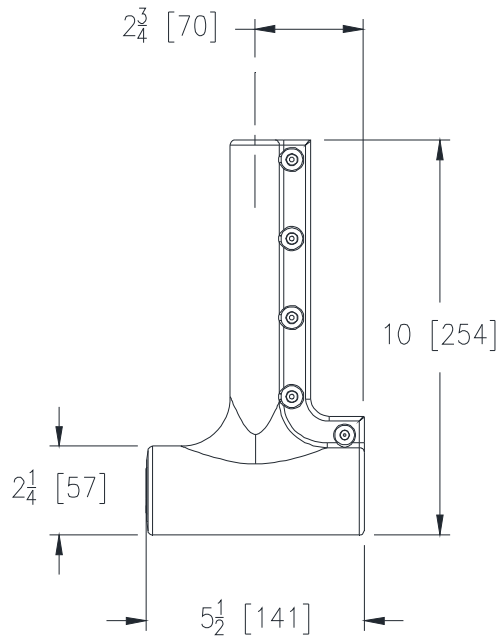
SUPPLY STOP PROTECTOR
